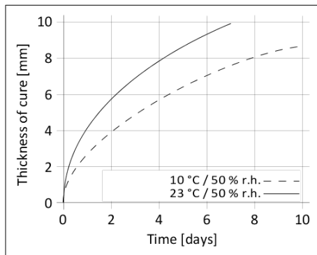
Diagram 1: Herdehastighet for SikaTack® PRO (Purform®)
